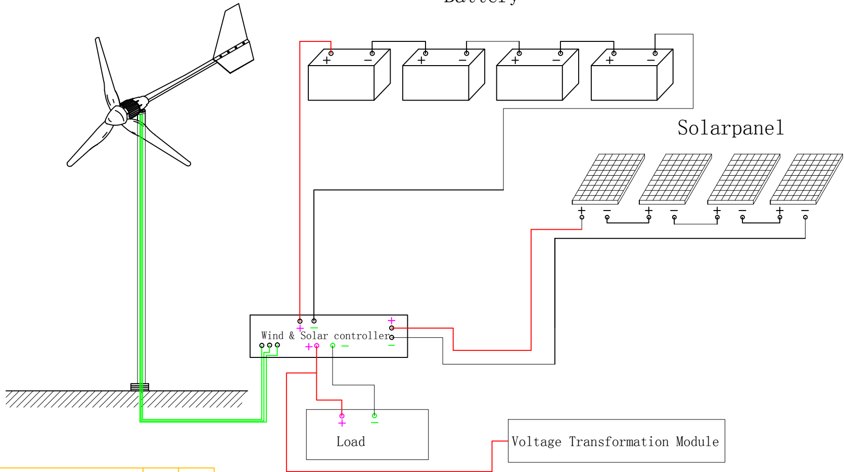
48V Wind & Solar System wiring Diagram
