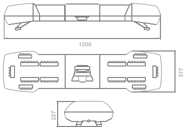
LBD-140013 | Lightbar
