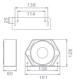
HA-102/152 | Hexangular Speaker
